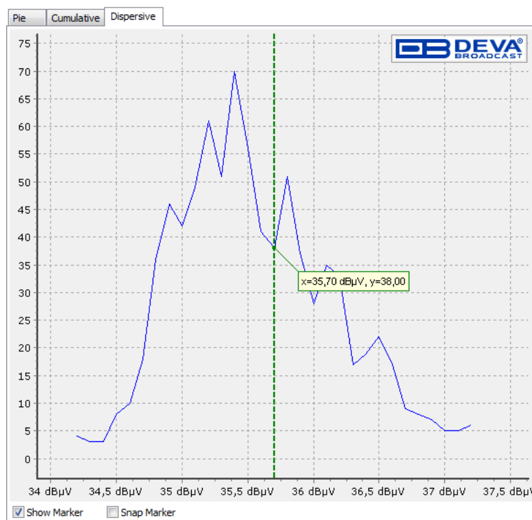
Dispersive
